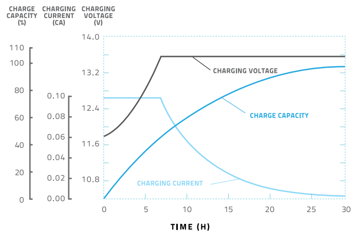
FLOATING CHARGE CHARACTERISTICS 77°F (25°C)
